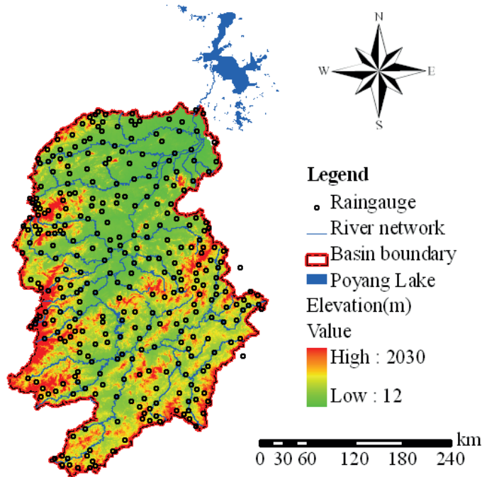
Fig. 1 Sketch map of the location of the study area and the rain gauges' distribution.
