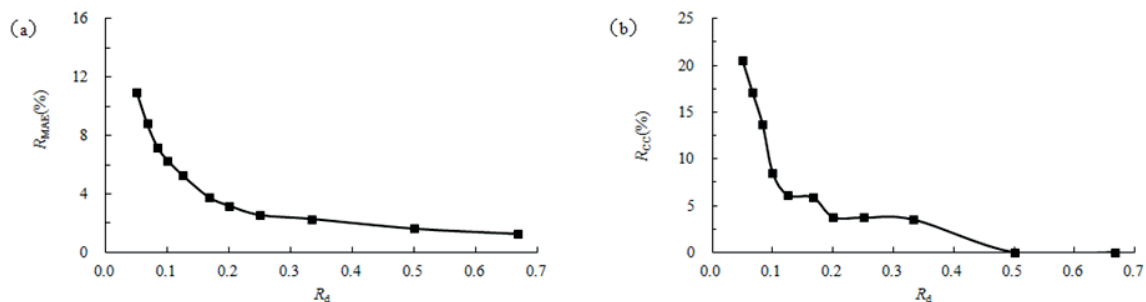
Fig. 2 R_{MAE} and R_{CC} under various scenarios of the calibration rain gauges relative to the total 325 in the Ganjiang River basin.
